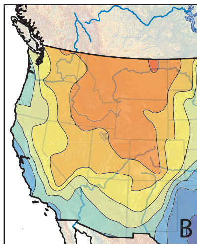
Fig. 2. (A) Map showing sample locations for stable isotopic studies presented in this paper. Symbols show the type of material analyzed for stable isotope values. Dots represent calcite from paleosols (Smith and others, 1993; Wang and others, 1993; Mack and others, 1994; Fox and Koch, 2004; Horton and others, 2004; Kent-Corson and others, 2006; Horton and Chamberlain, 2006; Fan and others, 2011; this study), paleolake sediments (Rogers and others, 1992; Poulson and John, 2003; Davis and others, 2008, 2009a, 2009b; this study) and fossil bivalves (Fan and Dettman, 2009); squares represent smectite from weathered ashes (Poage and Chamberlain, 2002; Takeuchi and Larson, 2005; Sjostrom and others, 2006); diamonds represent hydrated glasses from volcanic ashes (Mulch and others, 2008; Cassel and others, 2009b); triangles represent kaolinite from weathered stream deposits (Mulch and others, 2006); and pentagons are muscovite from shear zones (Mulch and others, 2004, 2007). (B) Modern \delta^{18}\text{O} values for surface waters, from Kendall and Coplen, 2001.
